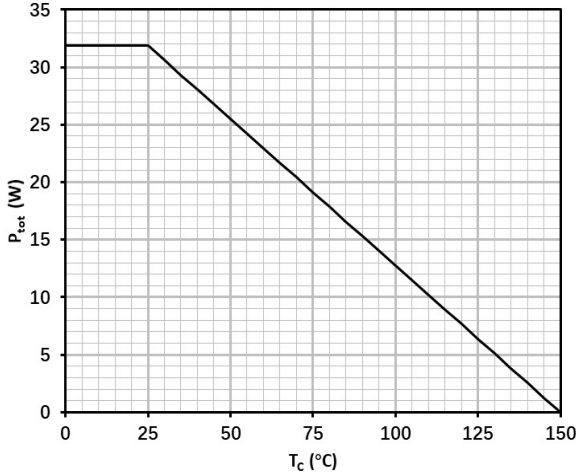
Figure 14 Power dissipation
